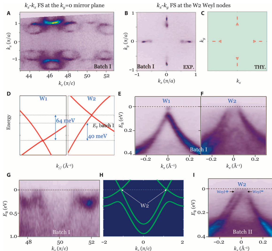
Fig. 2. Bulk Weyl fermion cones in TaP. (A) SX-ARPES Fermi surface (FS) map at k_y = 0 in the k_z - k_x plane. (B) SX-ARPES Fermi surface map at k_z = W2 in the k_x - k_y plane, showing the W2 Weyl nodes. EXP, experimental. (C) Theoretical calculation of the same slice of the BZ at the same energy shows complete agreement with the SX-ARPES measurement. THY, theoretical. (D) First-principles calculations of the energy-momentum dispersion of the two sets of Weyl nodes, W1 and W2, in TaP. The two nodes are offset in energy by 64 meV. (E and F) Energy dispersion maps, E - k_{\parallel} , for W1 and W2, respectively. (G and H) ARPES measured and theoretically calculated out-of-plane dispersion, E - k_z , for W2, which shows the linear dispersion of the Weyl cone along the out-of-plane direction. All data in (A) to (G) are obtained from Batch I. (I) Energy dispersion of the W2 Weyl cones from a sample in Batch II. We see the \pm Weyl nodes more clearly for Batch II TaP, as labeled in (I).
