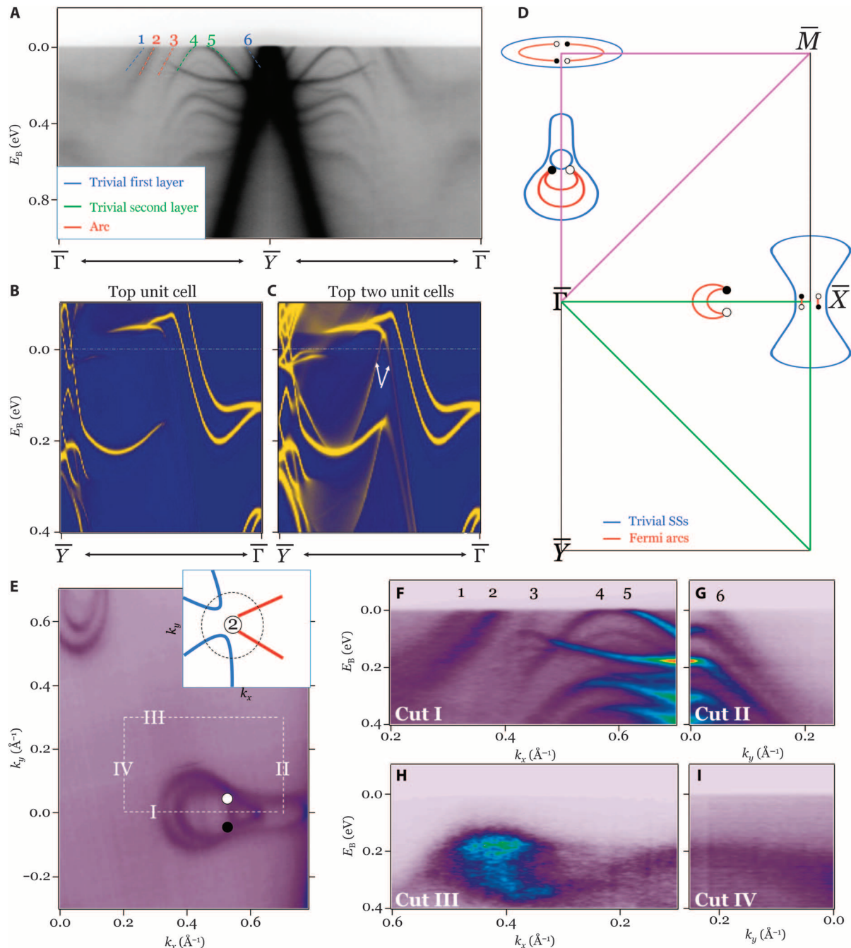
Fig. 4. Bulk-boundary correspondence and topological nontrivial nature of TaP. (A) ARPES energy-momentum dispersion map along the \bar{\Gamma} - \bar{Y} - \bar{\Gamma} high-symmetry line, which shows six band crossings at the Fermi level. (B) Calculated energy dispersion along the \bar{Y} - \bar{\Gamma} line. The calculation uses the Green function technique to obtain the spectral weight from the top unit cell of a semi-infinite TaP system. (C) Similar to (B) but for the top two unit cells. (D) Schematic examples of closed paths (green and magenta triangles) that enclose both W1 and W2 Weyl nodes. The bigger black and white circles represent the projected W2 nodes, whereas the smaller ones correspond to the W1 nodes. The red lines denote the Fermi arcs and the blue lines show the trivial surface states. The specific configuration of the surface states in this cartoon is not intended to reflect the Fermi arc connectivity in TaP. It simply provides an example of one configuration of the surface states that is allowed by the projected Weyl nodes and their chiral charges by the bulk-boundary correspondence. (E) Zoomed-in ARPES spectra near the W2 nodes along \bar{\Gamma} - \bar{Y} . The white dashed line marks a rectangular loop that encloses a projected W2 Weyl node. The circles are added by hand on the basis of the calculated locations of the projected W2 nodes. (F to I) ARPES dispersion data as one travels around the k -space rectangular loop shown in (E) in a counterclockwise way from I to IV. The closed path has edge modes with a net chirality of 2, showing that the path must enclose a projected chiral charge of 2 using no first-principles calculations, assumptions about the crystal lattice or band structure, or ARPES spectra of the bulk bands.
